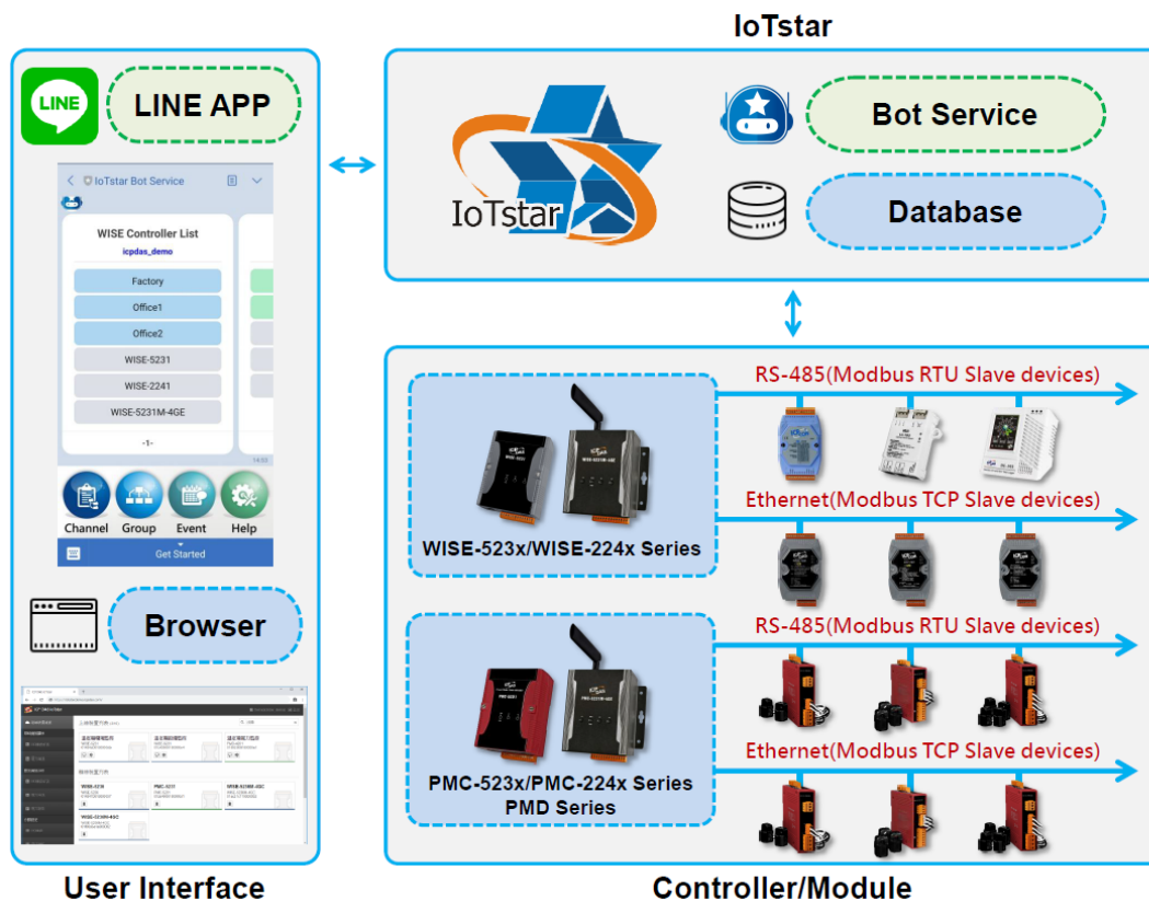
Figure 1-2: IoTstar 2025 Bot Service (LINE) System Architecture
